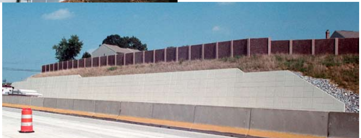
T-WALL® Retaining Wall System
