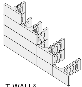
T-WALL® Retaining Wall System
